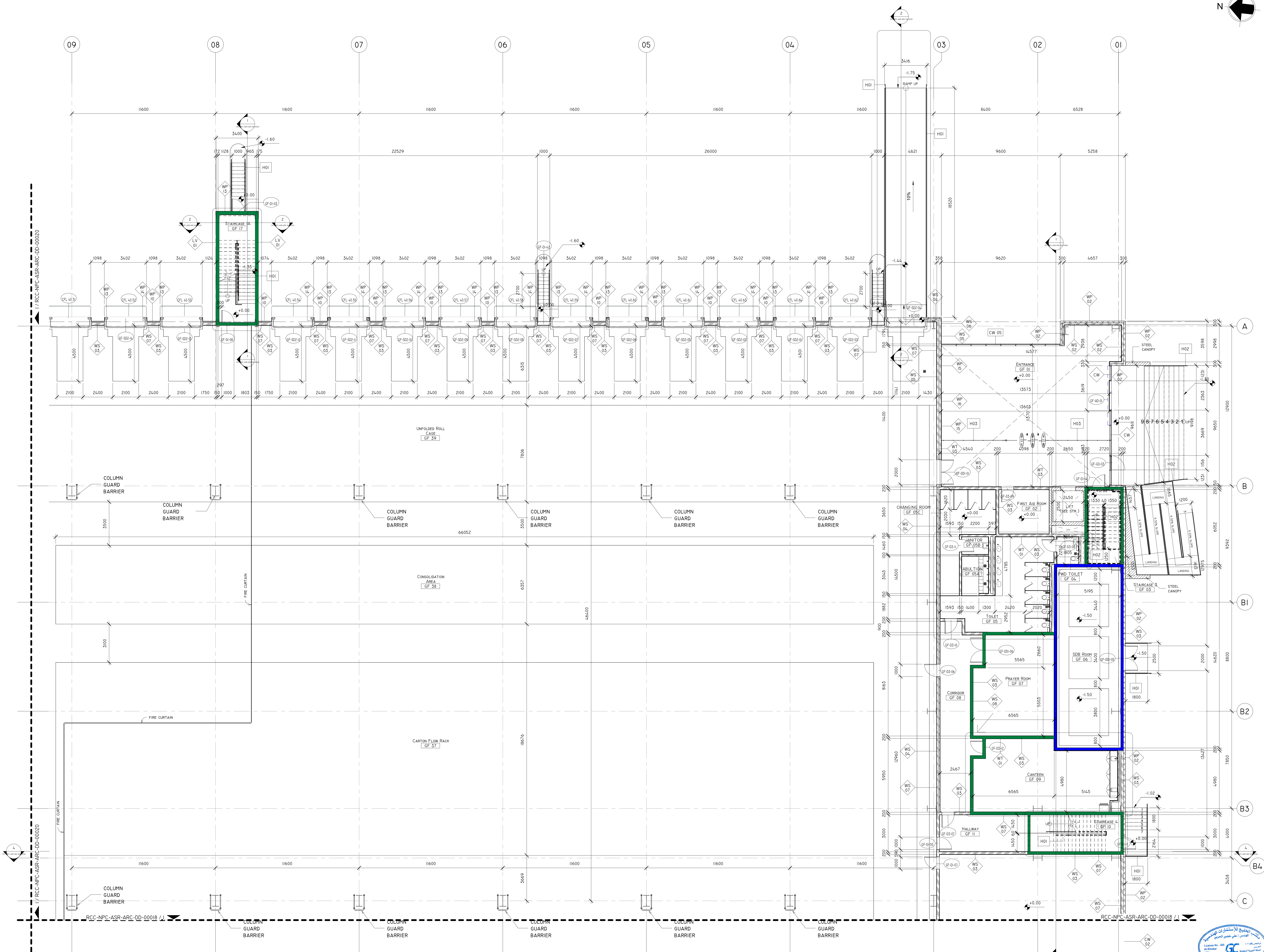
01- GROUND FLOOR GENERAL LAYOUT - PART A 1 : 100
